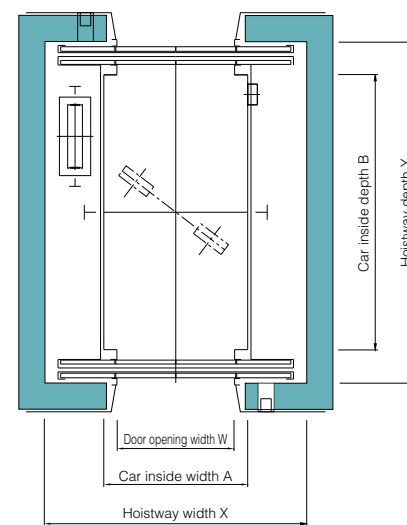
Front and rear opening hoistway plan (Type: P13D2)
