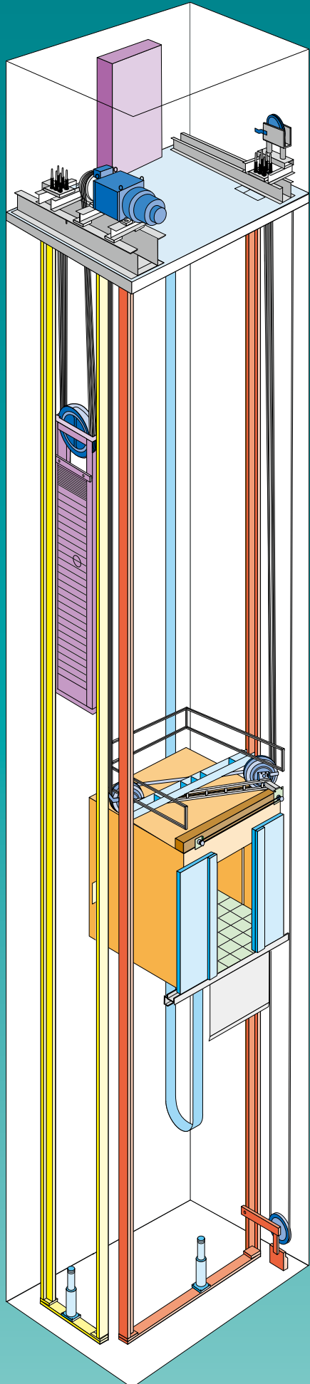
System image (Counterweight at side location type)
