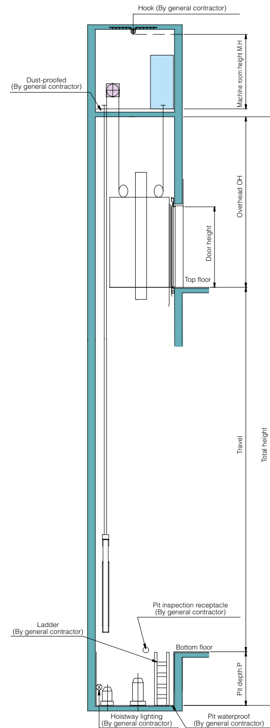
Hoistway section
