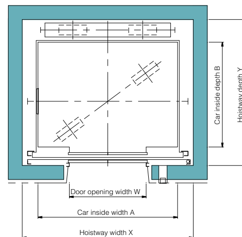
Hoistway plan
