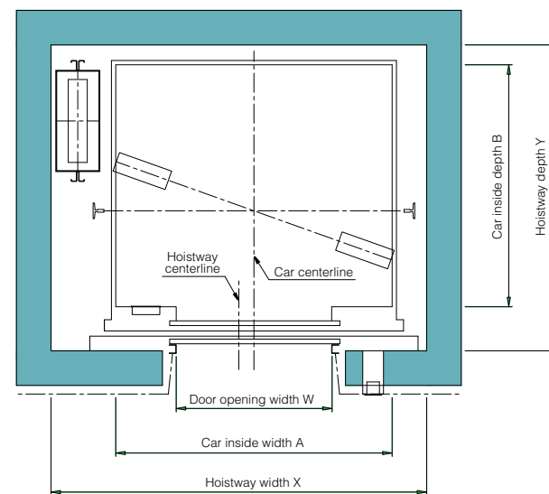
Hoistway plan
