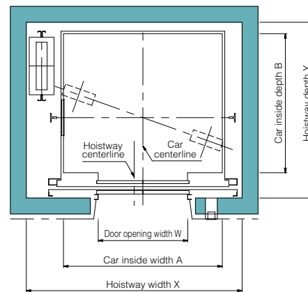
Center opening door hoistway plan (Type: P15W)
