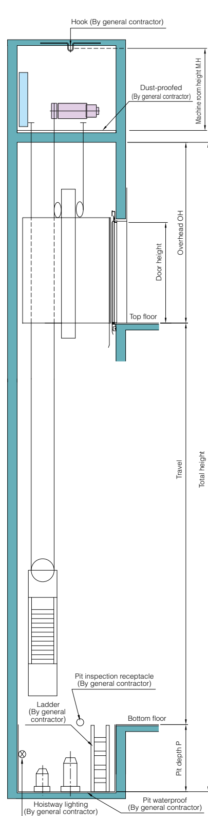
Hoistway section
