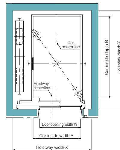
Two panel side door hoistway plan (Type: P17D, P21D)
